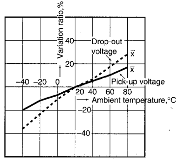
9. Ambient temperature characteristics Tested sample: TQ2-12V, 5 pcs.
